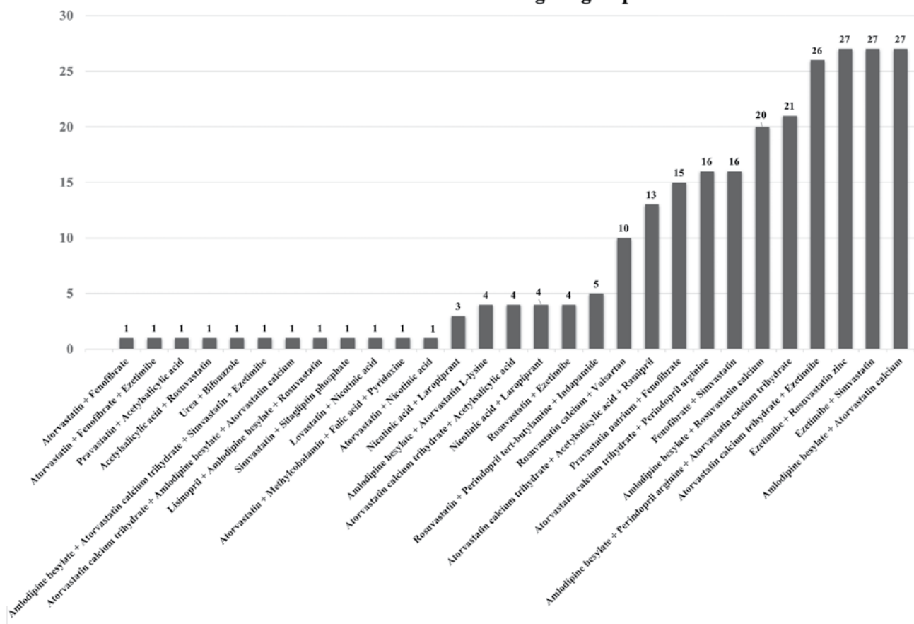
Fig. 2. Diagram of the ratio of combined drugs of group C10
